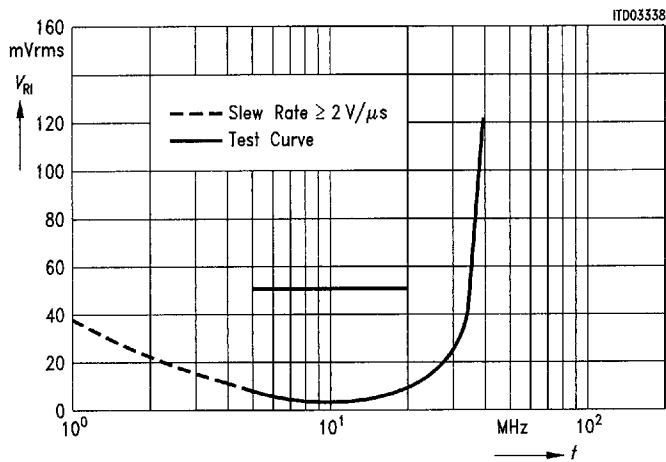
Diagram 24 Input Sensitivity (typ.) of RI Input T_A = 25\text{ }^{\circ}\text{C} , V_{DD} = 3\text{ V}
