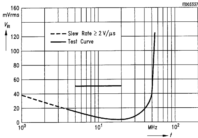
Diagram 23 Input Sensitivity Single Modulus (typ.) of FI Input T_A = 25\text{ }^{\circ}\text{C} , V_{DD} = 3\text{ V}
