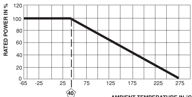
Derating
